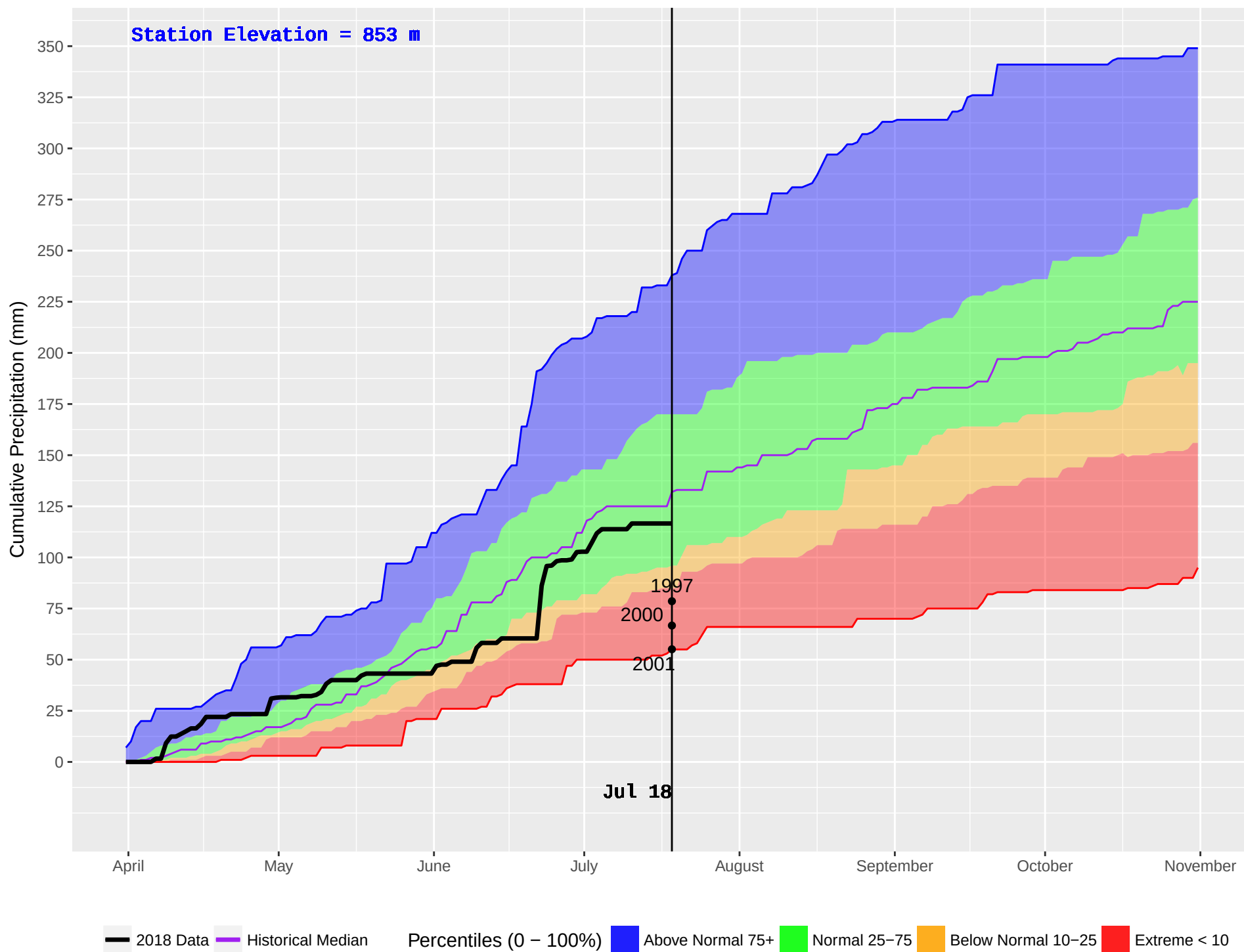
JOHNSON LAKE (419) : Historical (1986–2016) and Current (2018) Daily Cumulative Precipitation
